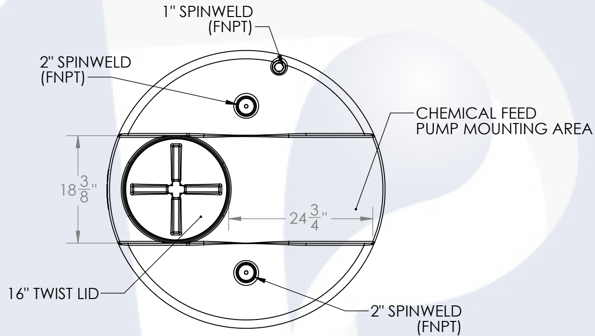
PLAN VIEW
